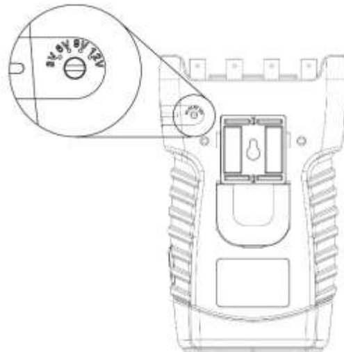
Figure 3-3. Power out voltage selector
